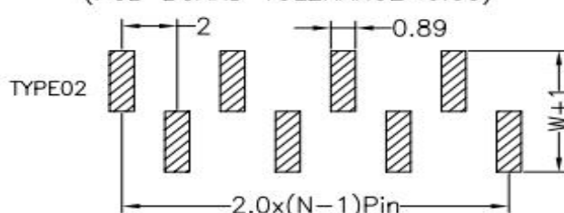
Recommended P.C.B Layout(Top Side) (PCB BOARD TOLERANCE±0.05)
