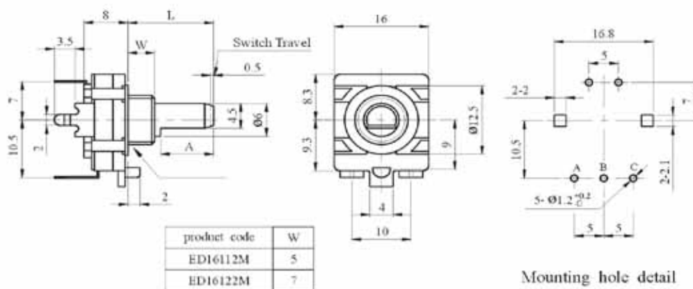
Mounting hole detail
