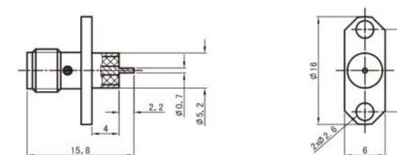
SMA-50KFD21
