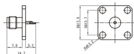
SMA-50KFD50
