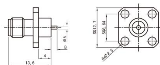
SMA-50KFD42
