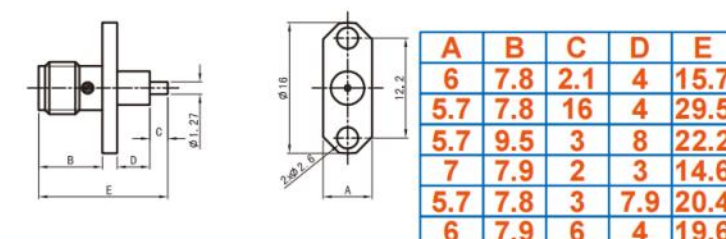
SMA-50KFD56
