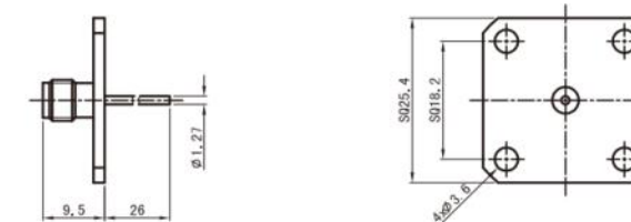
SMA-50KFD21
