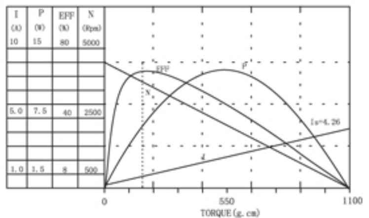
DRC-555PH-2670 12VDC
