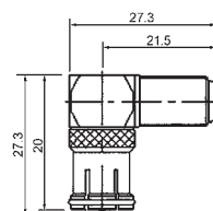
M56431 Double F female bulkhead (F-81)
