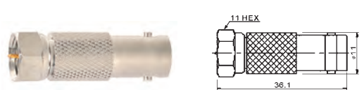
M5613 F male to BNC female gold-pin
