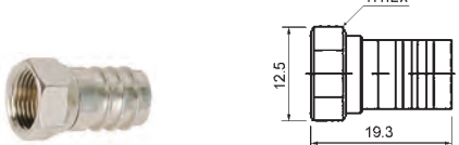
M5609 F male twist on type (RG58U/59U/5C2V)
