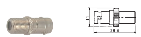
M5620 F female to BNC female gold-pin
