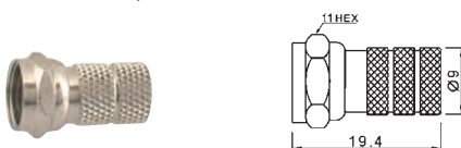
M5609 F male twist on type (RG58U/59U/5C2V)
