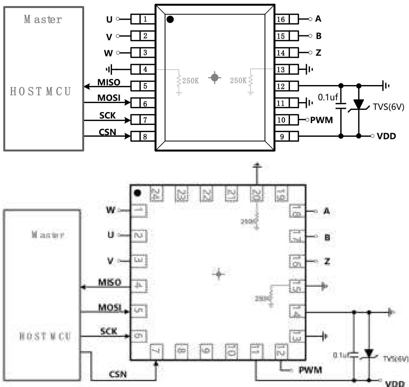
Figure 6: Reference Circuit without User Auto-Calibration
