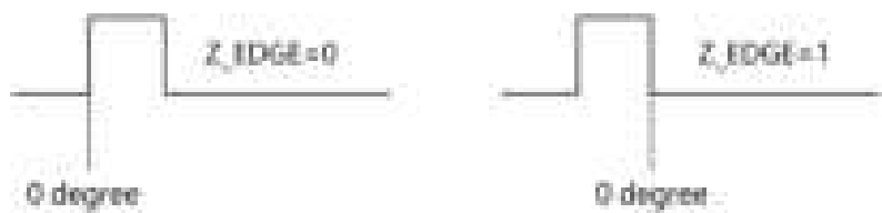
Figure 14: Z Pulse Edge with 0 degree
