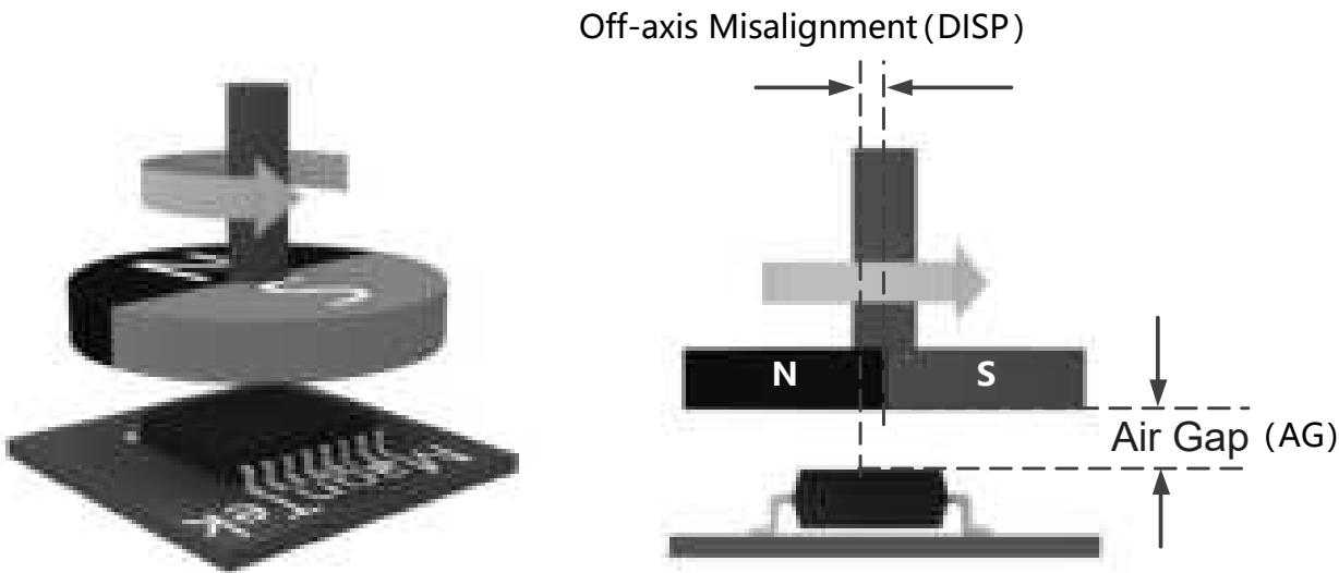
Figure 5: Magnet Arrangement
