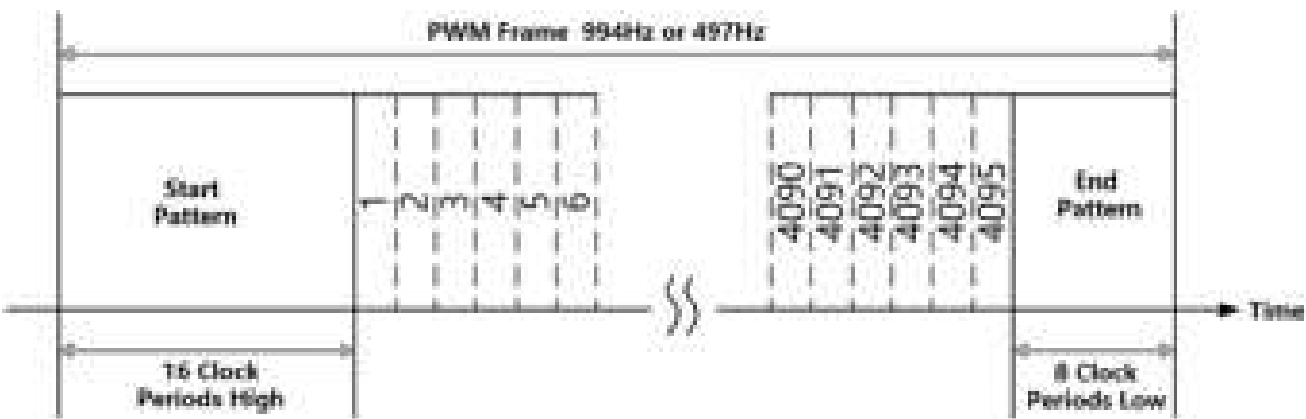
Figure 16: PWM Output Frame
