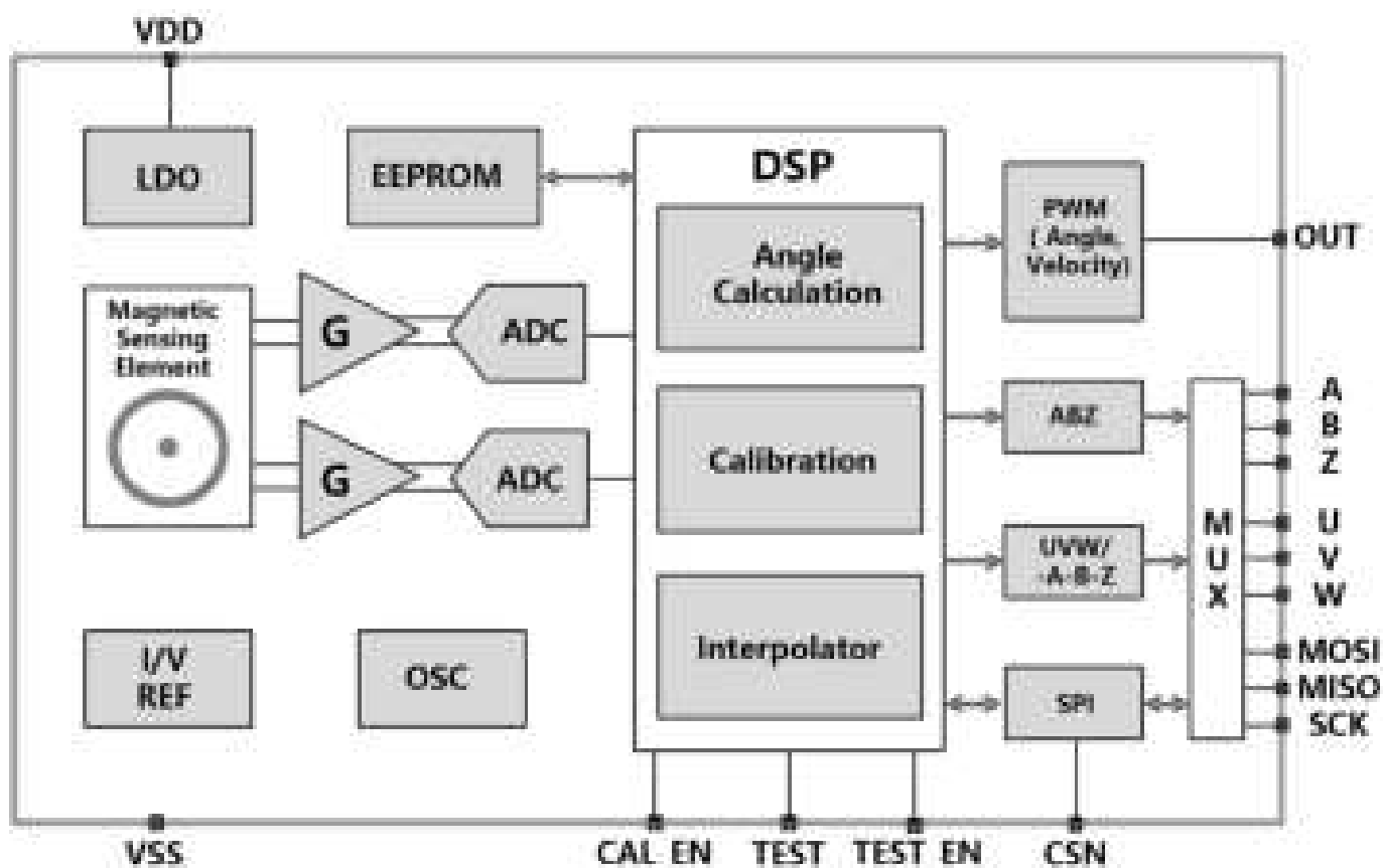
Figure 3: Block Diagram
