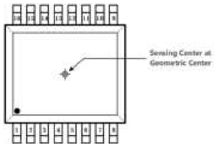
Figure 1: Pin Configuration of MT6826S (TSSOP-16) Package
