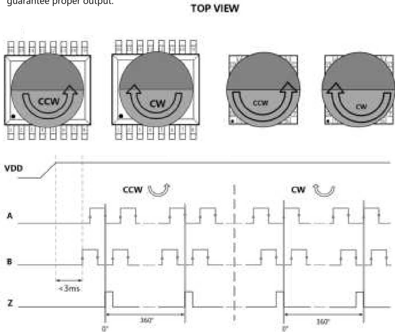
Figure 8: ABZ output with VDD power on
