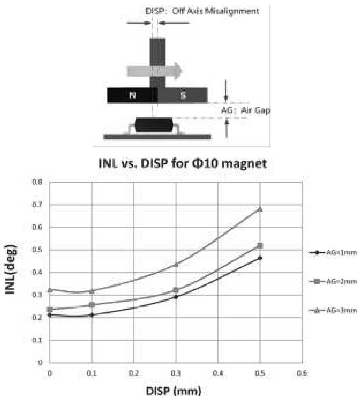
Figure 30: INL vs DISP and AG with Factory Calibration Only
