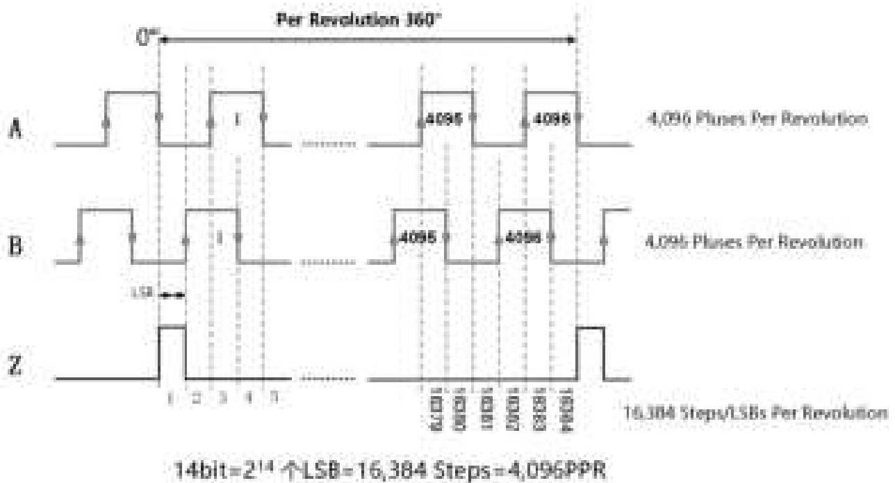
Figure 9:ABZ Output Resolution=14bit=4,096PPR
