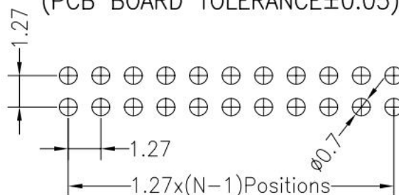
Recommended P.C.B Layout(Top Side) (PCB BOARD TOLERANCE±0.05)
