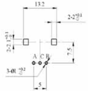
Mounting hole detail
