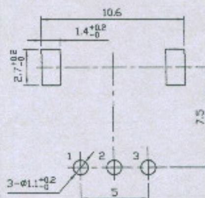
PCB TERMINAL POSITION
