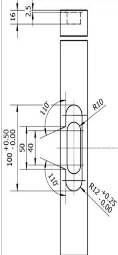
Hole Dimension on the Door Frame
